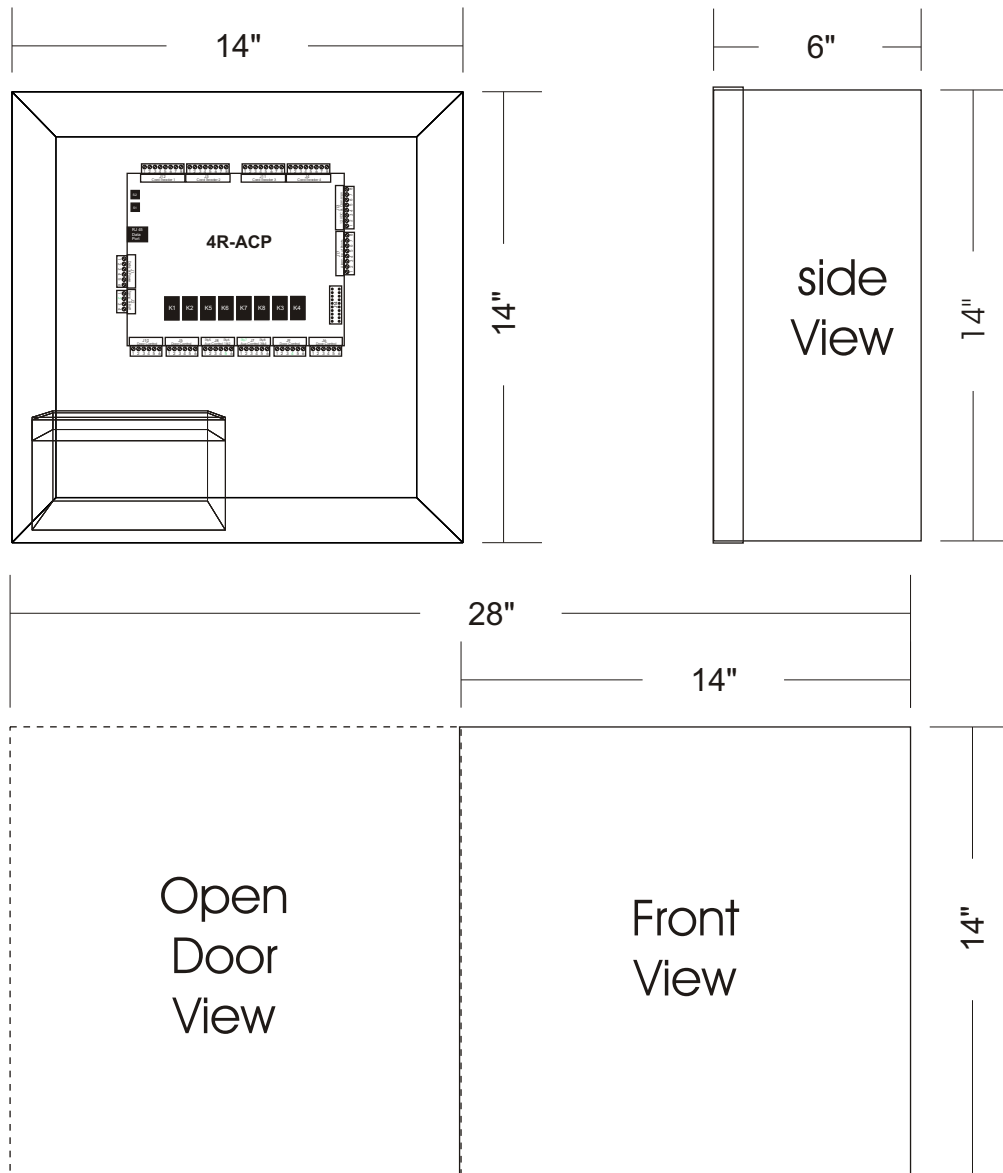
4R-ACP 4-Reader Control Panel Back box Space Requirements
